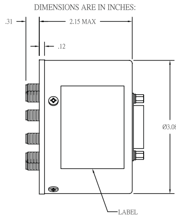
11X SMA FEMALE CONNECTORS 10X EQUALLY SPACED ON A Ø1.740 [Ø44.20] B.C.
