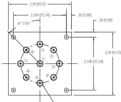
9X SMA FEMALE CONNECTORS 8X EQUALLY SPACED ON A Ø1.540 [Ø39.12] B.C.
